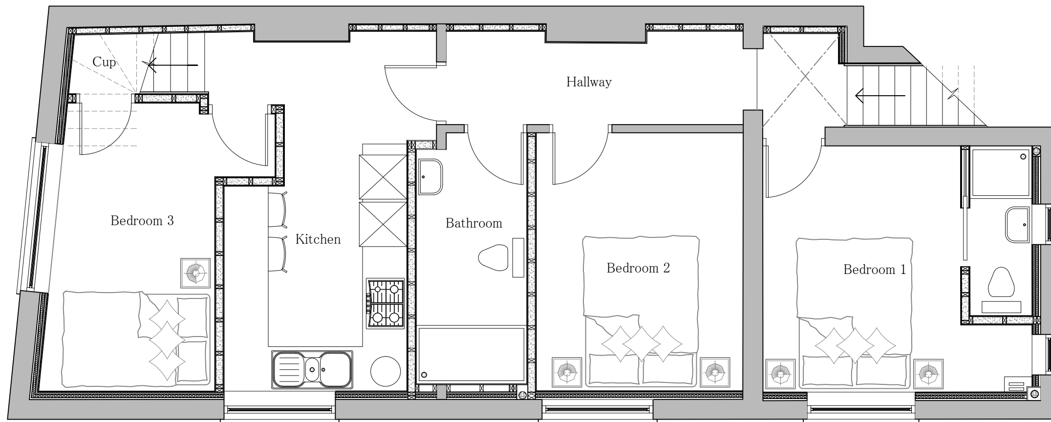
PROPOSED FIRST FLOOR FLAT @ 1:50
